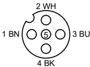
Female M12
