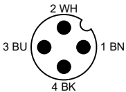
Male M12
